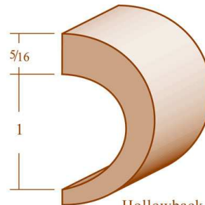
Hollowback Landing Strip 522 7/16 x 1 5/8
