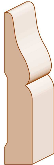
Moulded Base 2246 * \frac{5}{8} \times 3\frac{1}{2}
