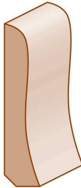
Cove Base 336 \frac{3}{8} \times 1\frac{7}{8}
