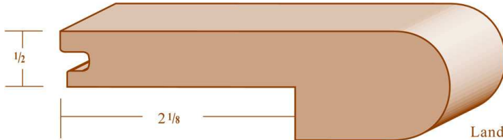
Landing Strip 7772 * 1 x 3 1/2
