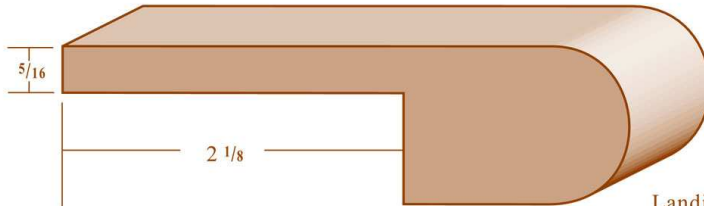
Landing Strip 7770 * 1 x 3 1/2
