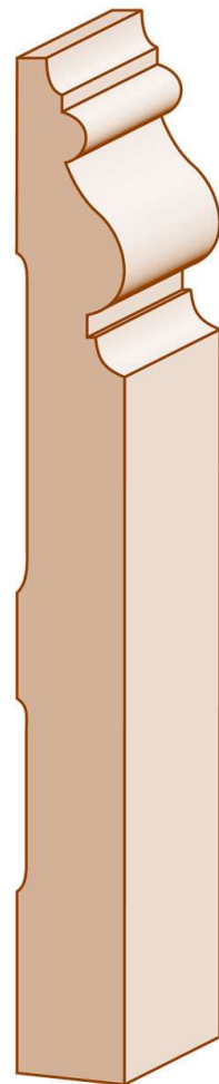
Base 2232 * \frac{9}{16} \times 5\frac{3}{8}
