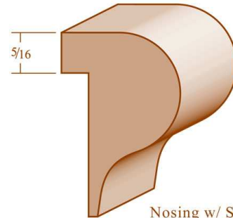
Nosing w/ Scotia 534 1 1/16 x 1 5/16
