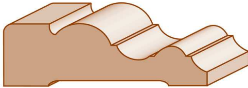
Casing 1134 * \frac{3}{4} \times \frac{27}{16}
