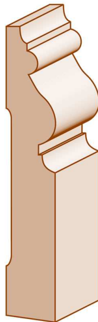
Base 2230 * \frac{9}{16} \times 3\frac{3}{8}
